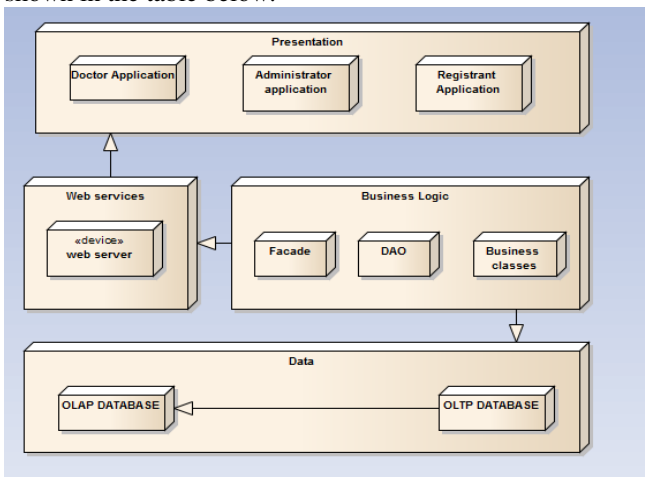
Figure 4 : Deployment Diagram
